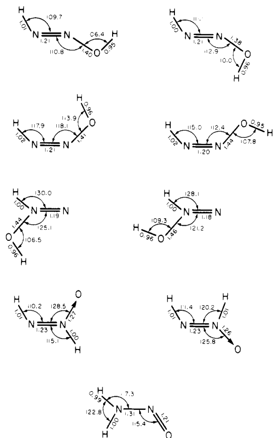
Figure 1. Optimized geometries for \text{N}_2\text{H}_2\text{O} isomers. Angles in degrees and distances in Ångstroms.
