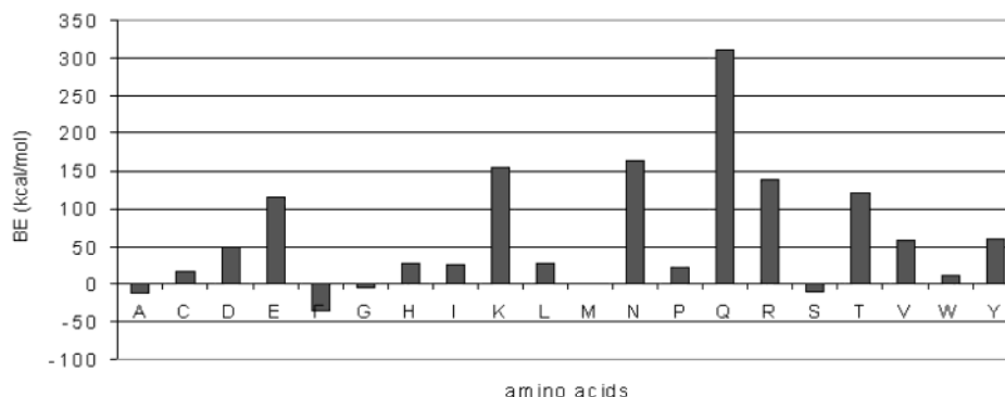
Figure 10. Binding energies of 20 amino acids using the conformations generated from perturbation of the Phe binding site in PheRS.
