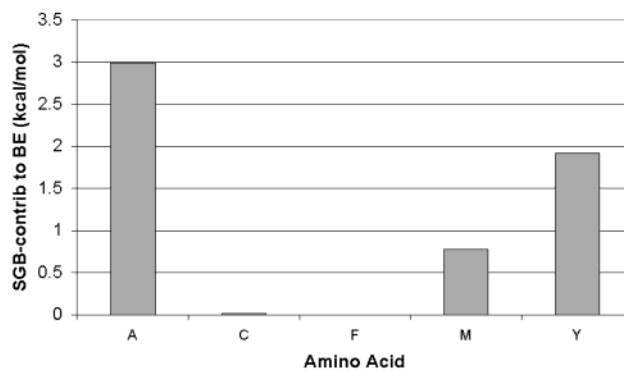
Figure 7. Relative reduction of ligand binding energy due to differential solvation (SGB). F is taken as the reference. Note that A and Y are especially excluded by this term.
