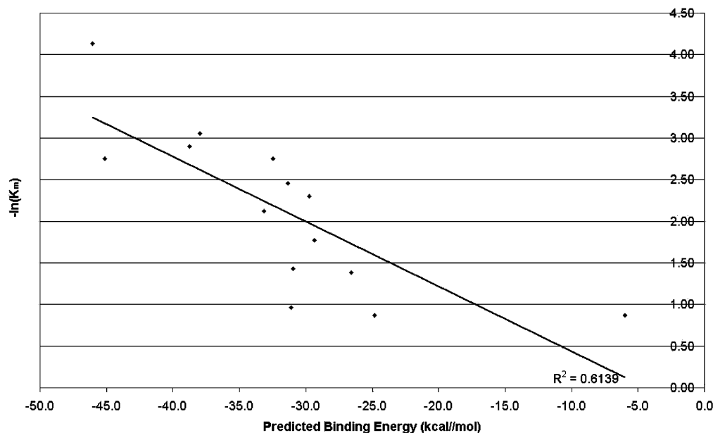
Figure 8. Comparison of the experimental K_m values (310 K) for the 13 neutral amino acids to PheRS determined by Friest 36 with the predicted binding energies (0 K) from HierDock. The R^2 of 0.61 goes to 0.68 if the Gly point is excluded. Note, the experimental values are for S. cerevisiae , while the predictions are for T. thermophilus .
