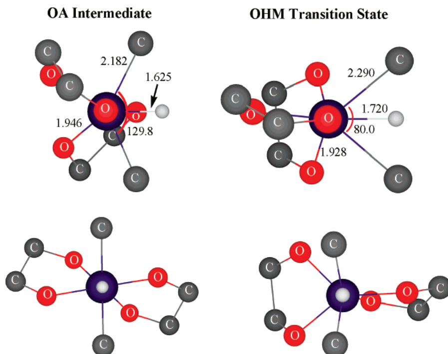
Figure 5. Geometrical configurations of secondary OA intermediate and OHM transition state for the (gly) 2 Re system. The spectator hydrogens have been removed for clarity. A few key bond distances (Å) and bond angles (deg) are shown. Note the dramatic conformational change the glycols make. Two different configurations are presented to clarify the extent of geometrical perturbation between the intermediate and the transition state.
