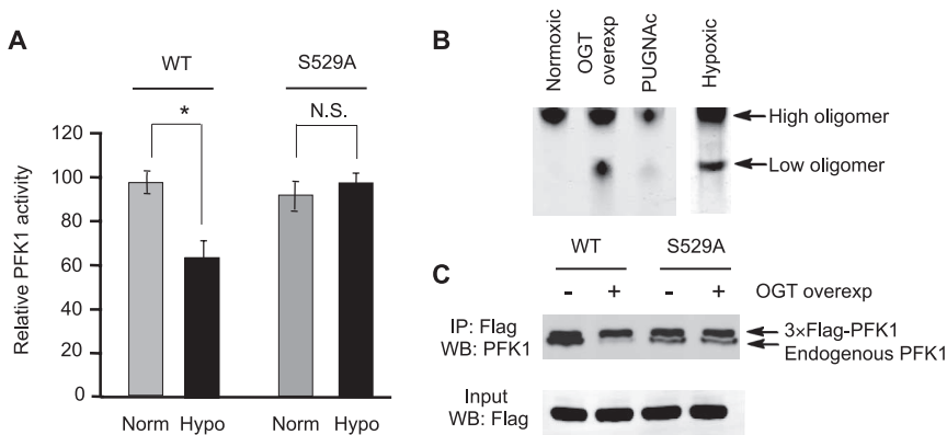
Fig. 2. Inhibition of PFK1 activity and oligomerization by glycosylation. (A) Relative activities of WT and S529A PFK1 (L isoform) purified from transfected 293T cells under normoxic or hypoxic conditions. Activities were measured in the presence of 100 μM F-2,6-BP and 3 mM ATP and were normalized with respect to the activity of WT PFK1 under normoxic conditions ( n = 3 assays). (B) Oligomerization state of Flag-tagged PFK1 (L isoform) purified from 293T cells under normoxic or hypoxic conditions and from 293T cells overexpressing OGT or treated with PUGNAc under normoxic conditions. Complexes were resolved by non-reducing SDS–polyacrylamide gel electrophoresis (SDS-PAGE) and visualized by Coomassie blue staining. (C) Coimmunoprecipitation (IP) of endogenous PFK1 with Flag-tagged WT or S529A PFK1 (L isoform) after OGT overexpression. Complexes were immunoprecipitated with a Flag antibody conjugated to agarose beads and analyzed by reducing SDS-PAGE, followed by immunoblotting with a PFK1 antibody. Error bars denote SEM. Statistical analysis was performed by Student's t test (* P < 0.05).
