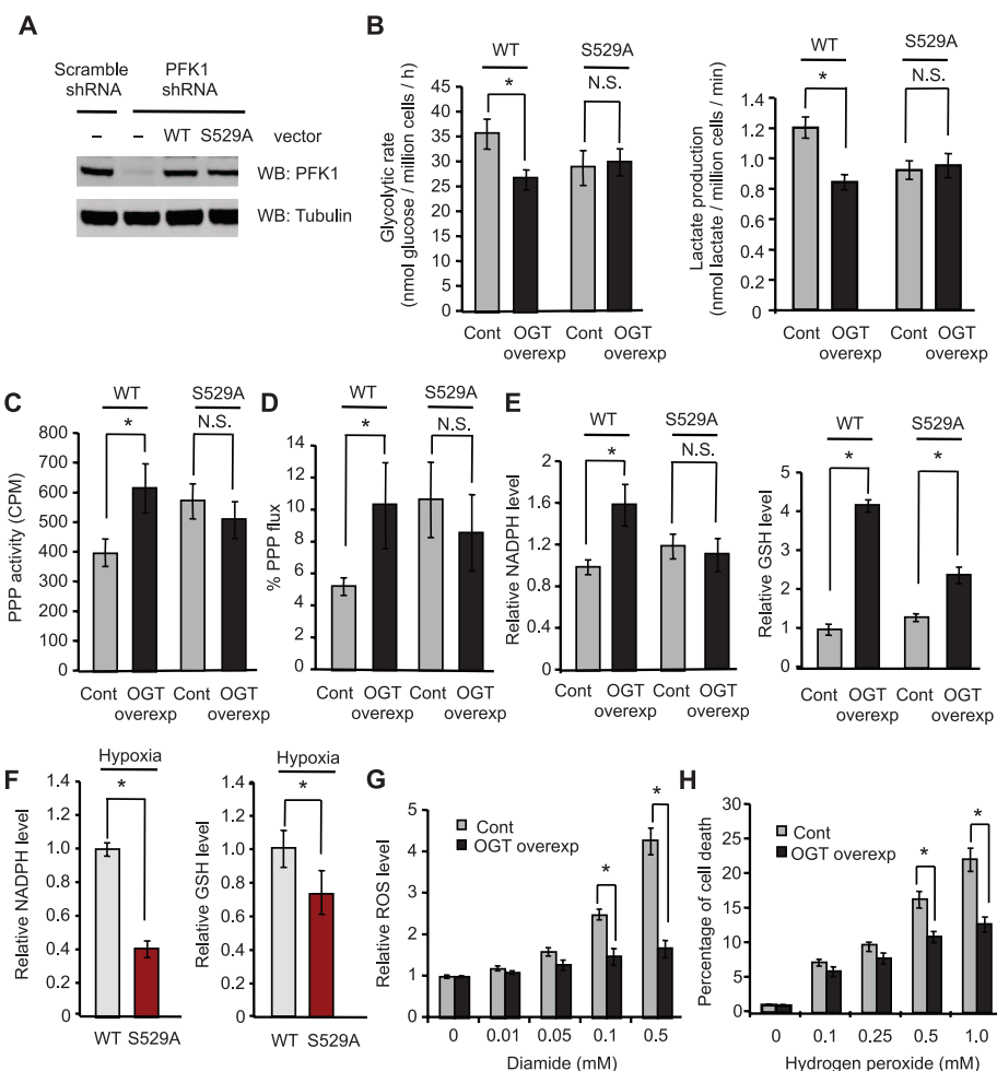
Fig. 3. PFK1 glycosylation at Ser 529 regulates glycolysis, increases PPP flux, and protects cells from ROS-mediated cell death. (A) Immunoblotting of H1299 cells stably expressing shRNA and rescue constructs. Flag-PFK1 levels were comparable to endogenous PFK1 levels. (B) Glycolytic rate and lactate production of H1299 cells rescued with WT or S529A PFK1 in the absence (Cont) or presence of OGT overexpression ( n = 4 experiments). (C) PPP activity in WT or S529A PFK1 rescue cells in the absence (Cont) or presence of OGT overexpression, as measured by the rate of 14 CO 2 production from glucose via the PPP ( n = 3 assays). (D) Percentage of central carbon flux from glucose to lactate flowing through the PPP in WT or S529A PFK1 rescue cells in the absence (Cont) or presence of OGT overexpression, as measured by reverse-phase triple-quadrupole liquid chromatography mass spectrometry. (E) NADPH and GSH levels in WT or S529A PFK1 rescue cells in the absence (Cont) or presence of OGT overexpression. NADPH and GSH concentrations are shown relative to WT PFK1 Cont and were assessed using a colorimetric assay and the thiol probe monochlorobimane, respectively ( n = 4 experiments). (F) NADPH and GSH levels in WT or S529A PFK1 rescue cells under hypoxic conditions ( n = 3 experiments). (G) Cellular ROS levels induced by varying concentrations of diamide in untreated H1299 cells (Cont) and H1299 cells overexpressing OGT, as measured by a fluorimetric assay. (H) Percentage of cell death induced by varying concentrations of hydrogen peroxide in untreated (Cont) and OGT-overexpressing H1299 cells, as measured by lactate dehydrogenase levels ( n = 4 assays). Error bars denote SEM. Statistical analysis was performed by Student's t test (* P < 0.05) for all figures.
